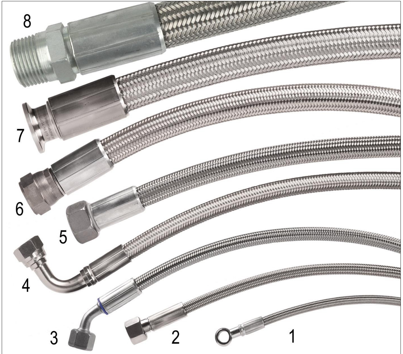
HYPERLINE SB Teflon hoses in stainless steel braid (AF-HDSB-...) with end fittings, crimped with sleeves AF-TH-... and AF-THU-...: 1 - DN5 (3/16") with lug TI-ZBB600-02-03; 2 - DN6 (1/4") with lug TI-ZMW121-16-04-SS304; 3 - DN8 (5/16") with 45° angle lug TI-ZMW321-16-05-CN; 4 - DN10 (3/8") with 90° angle nipple TI-ZBW210-06-06-SS; 5 - DN13 (1/2") with nipple TI-ZBW110-08-08-CN; 6 - DN16 (5/8") with nipple TI-ZJW110-14-10-CN; 7 - DN19 (3/4") with nipple hygienic stainless steel AF-FXXTC-034-16-019; 8 - DN25 (1") with TI-ZBZ130-16-16 end.
