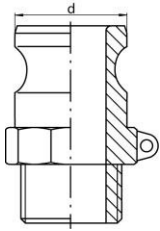
CAMLOCK connector plug with male thread BSPT or NPT
