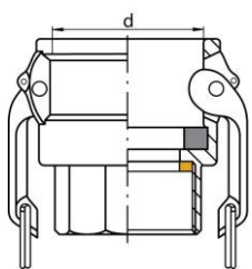
CAMLOCK connector socket with BSP female thread ISO-228-1
