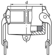
CAMLOCK connector plug blanking socket
