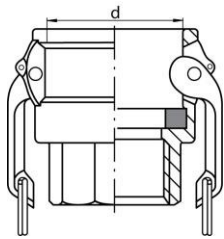
CAMLOCK connector socket with BSP or NPT female thread
