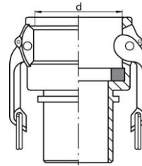
Socket for CAMLOCK connector with end for shell bracket EN 14420-3
