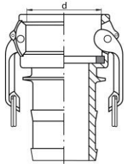
CAMLOCK connector socket with corrugated hose end
