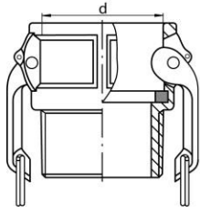
CAMLOCK connector socket with male thread BSPT or NPT
