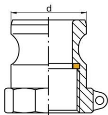
CAMLOCK connector plug with BSP female thread ISO-228-1
