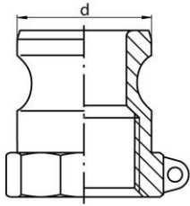
CAMLOCK connector plug with BSP or NPT female thread
